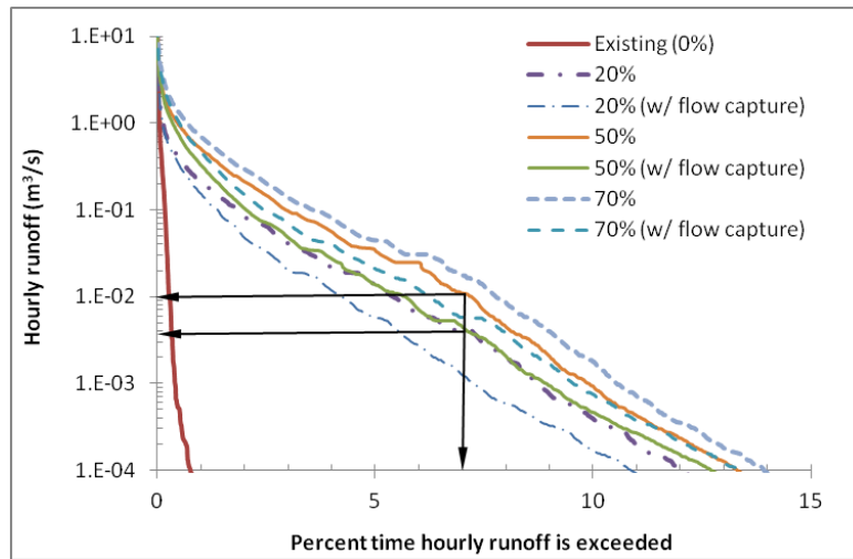
Figure 31. Effect of flow capture on flow duration curve for increasing TIA for Scrubby Creek. Plots for only 20, 50 and 70 percent TIA are shown for clarity.
