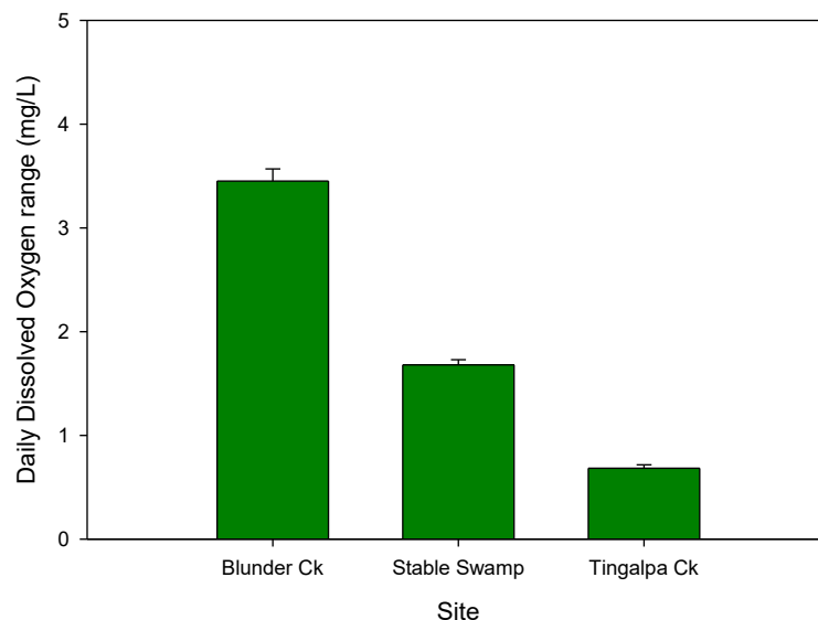
Figure 23. Mean daily dissolved oxygen range (mg/L) ( \pm SE) across all three sites for the period of record.
