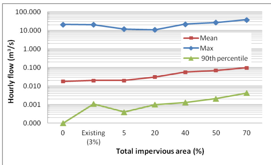
Figure 8. Modelled mean, max and 90 percentile hourly flow rate for different total impervious areas in Upper Yuan Creek catchment. The y axis is in log scale.
