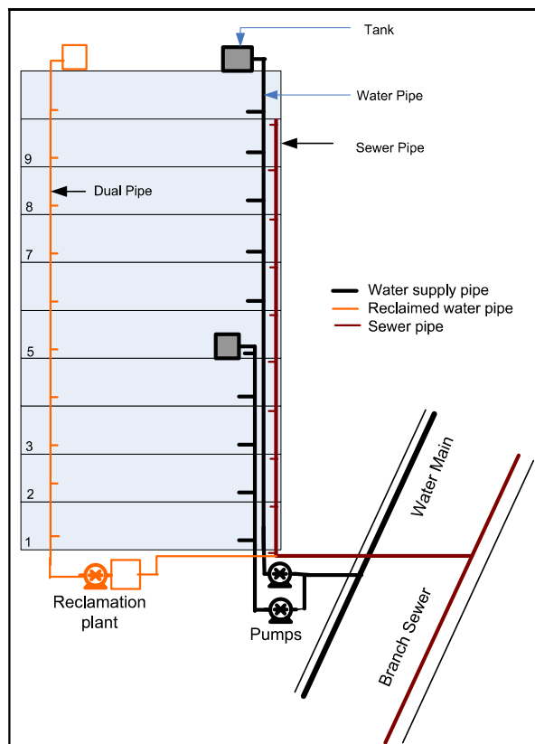
Figure 2: On-site wastewater system (Source: Sharma et al, 2005)
