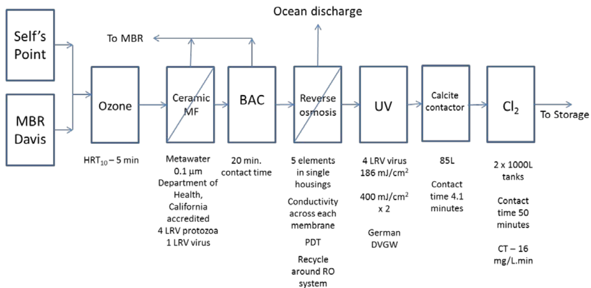
Figure 1: Schematic diagram of the AWTP Flowsheet
