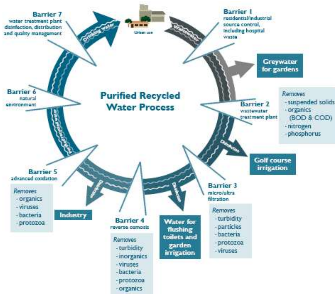
Figure 1 Schematic diagram of the Seven-Barrier treatment process employed in the WCRW Project (source: Queensland Water Commission Fact Sheet 4 1 )
