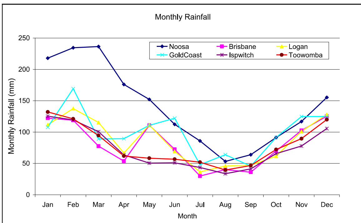
Figure 2: Monthly rainfall in some major cities of SEQ (1869–2008)
