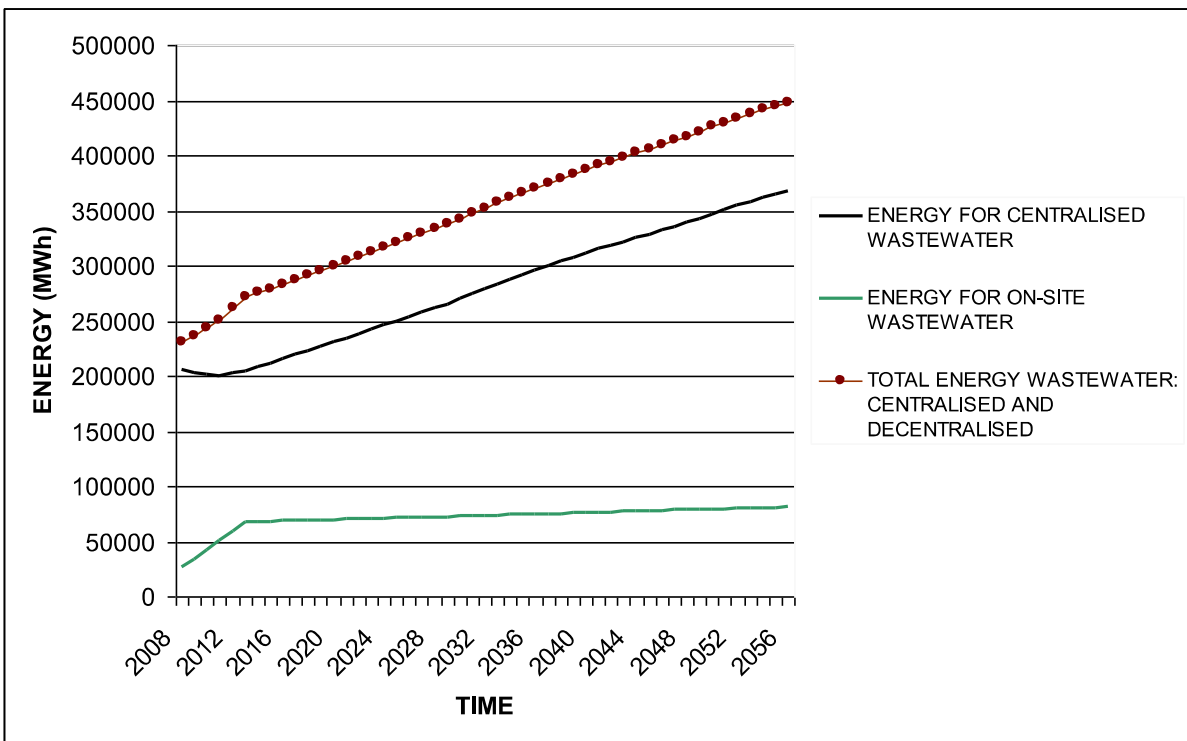
Figure 6: Draft predicted trend in total energy demand by centralised and decentralised wastewater management options (Hall et al. 2008)
