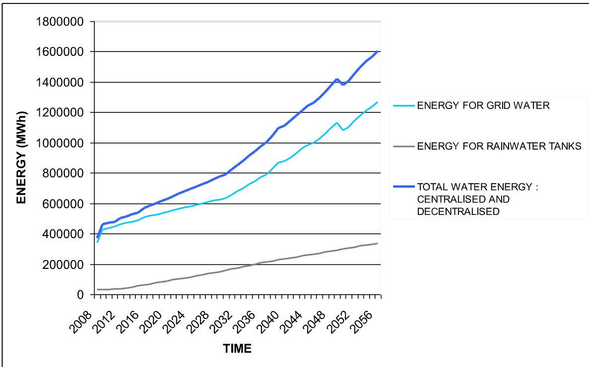
Figure 5: Draft predicted trend in total energy demand by centralised and decentralised water supply options (Hall et al. 2008)
